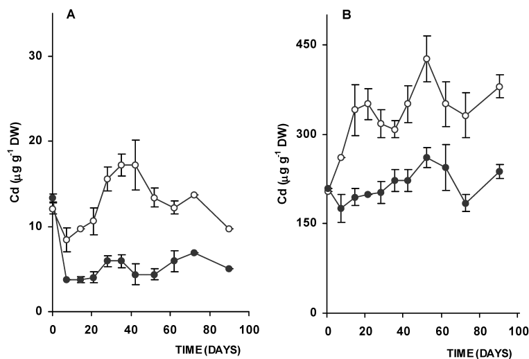
Figure 1. Extractable cadmium in the soil amended with CdO. A: Extracted with water; B: Extracted with \text{CaCl}_2 ; \circ — \circ : \gamma -Irradiated sterile soil; \bullet — \bullet : Native, non-sterile soil.
